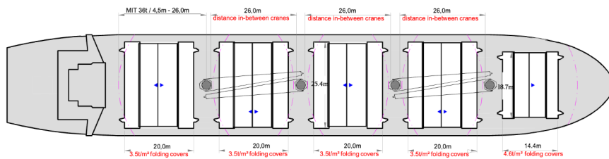
MAIN DECK
