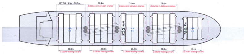
MAIN DECK
