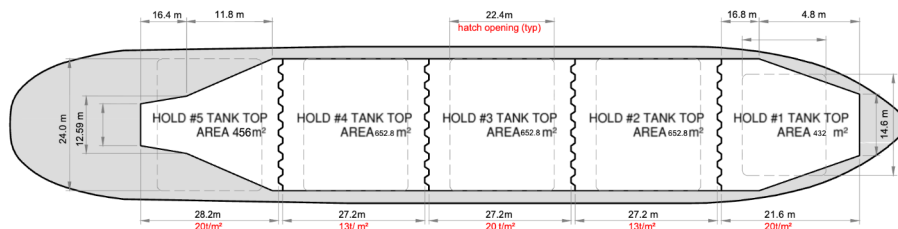
HOLDS & DOUBLE BOTTOM
