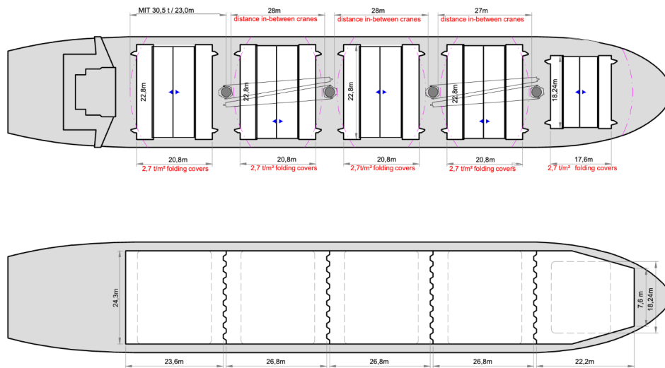
MAIN DECK
